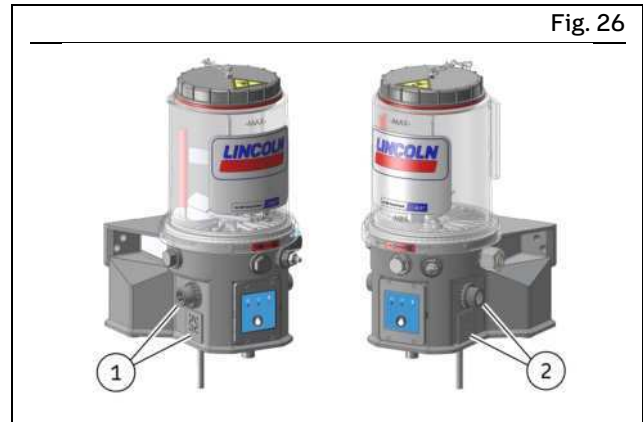
Electrical connection
