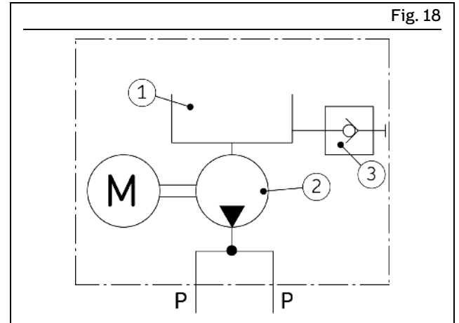
Pump without a follower plate
