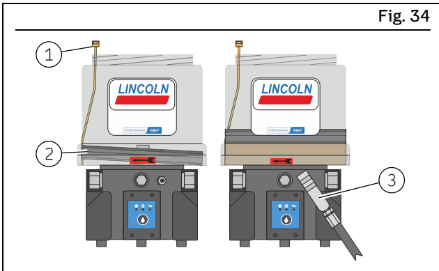
Inserting a cable tie and filling the pump
