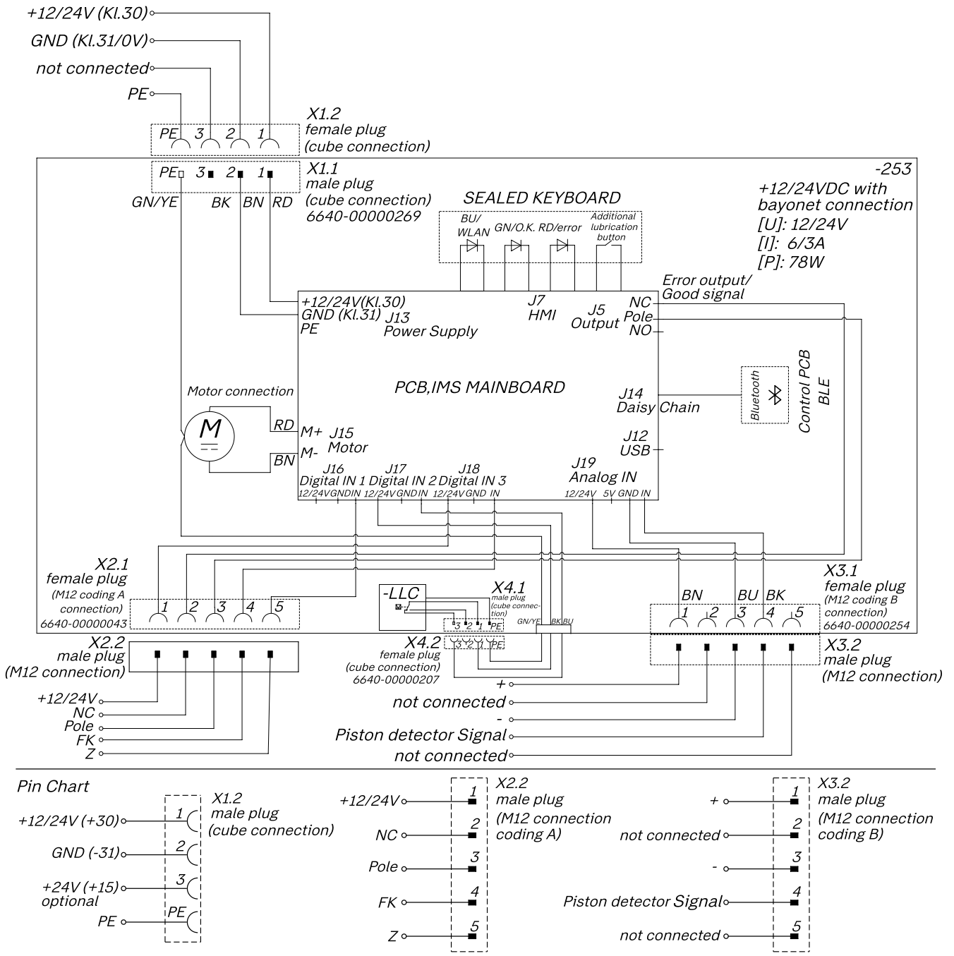
P253 DC Smart with rectangular connector and M12 socket (2x)
