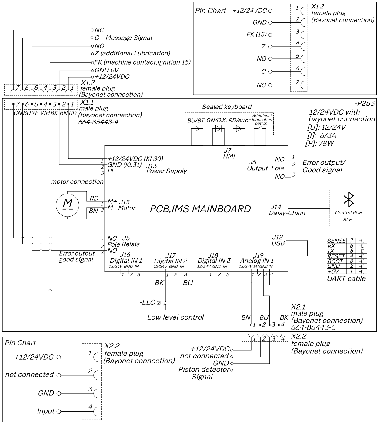
P253 DC Smart with bayonet connector (2x)
