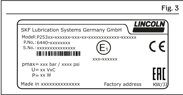
Type plate with ECE mark
