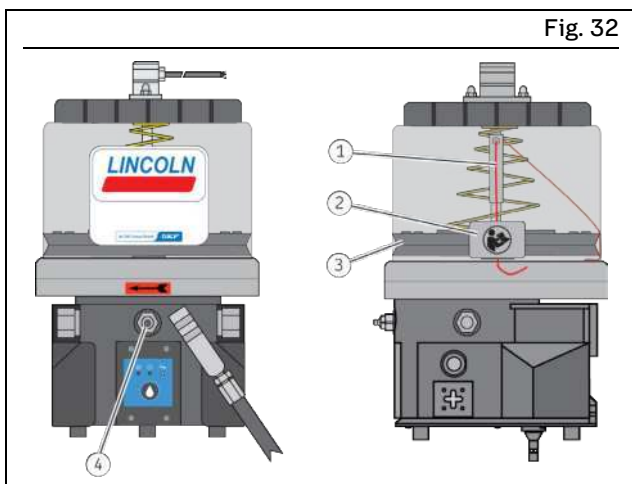
Initial filling
