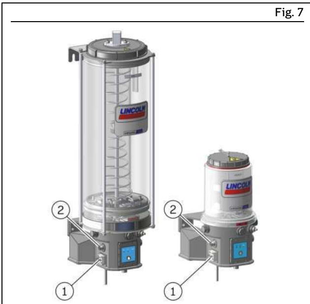
Electrical connections on the left
