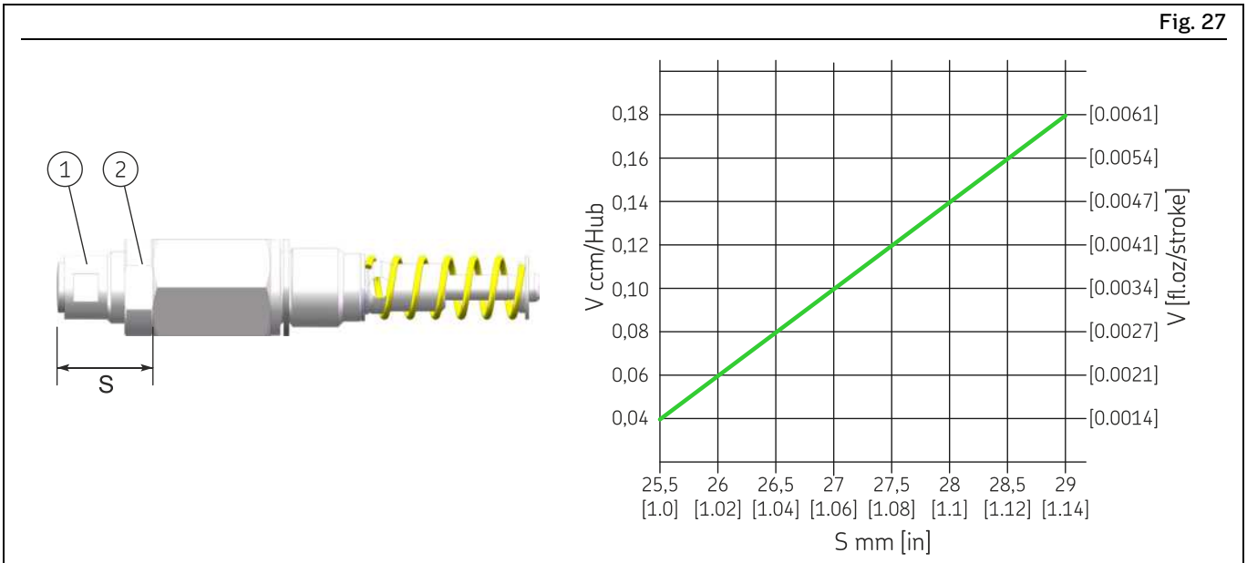
Setting the delivery rate on pump element R
