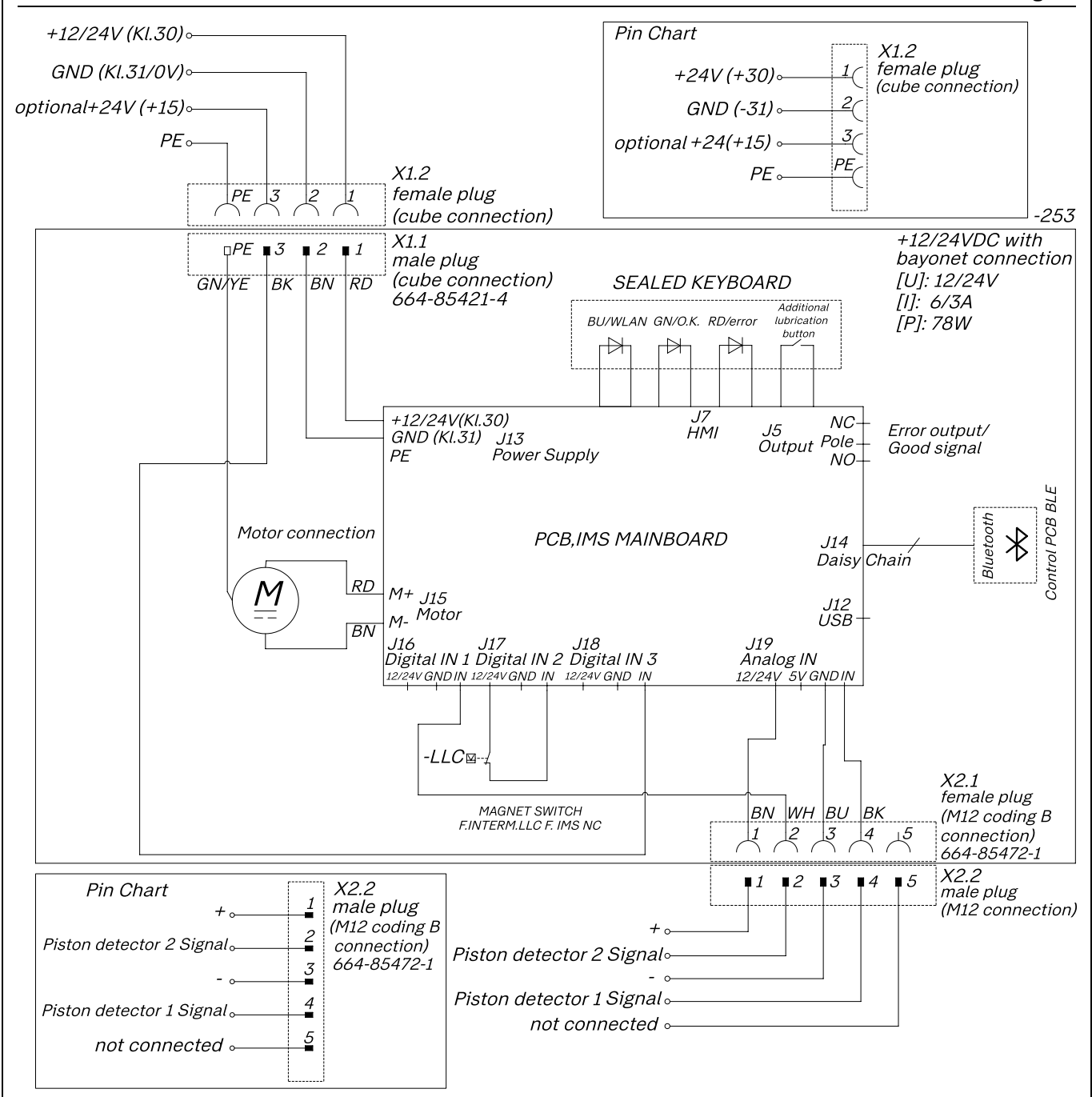
P253 DC Smart with rectangular connector and M12 socket
