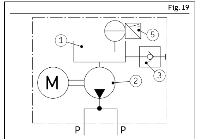
Pump without a follower plate and with low-level signal
