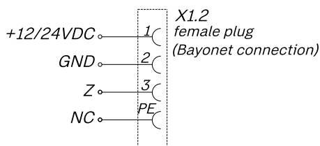
P253 DC Smart with bayonet connector (2x)
