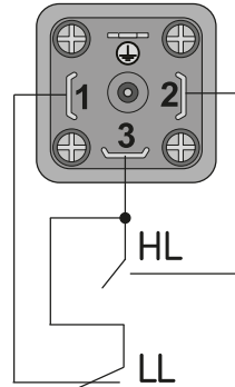
Connection diagram (lubrication grease) Reed switches for full and low-level signal
