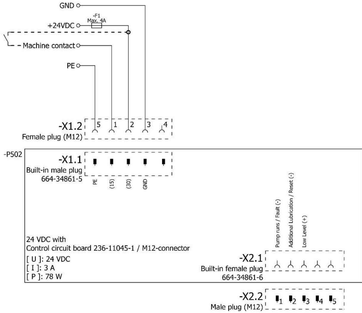
Terminal diagram 24 V DC with M12 connector and control circuit board V20
