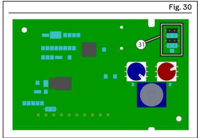
P502: setting jumpers for lubrication time and pause time
