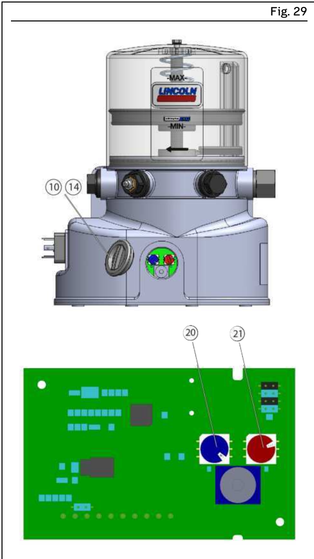
P502: Setting the lubrication time and pause time
