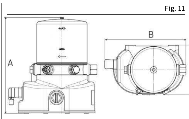
Mounting dimensions
