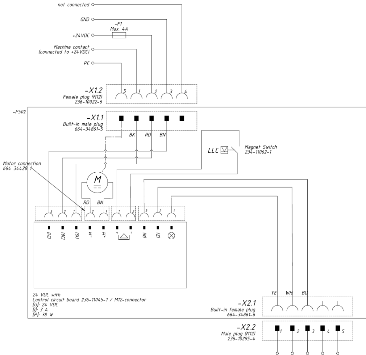
Terminal diagram 24 V DC with M12 connector and control circuit board
