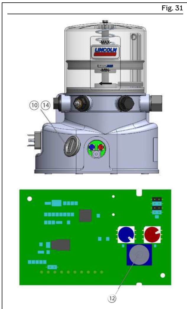
P502: Triggering additional lubrication
