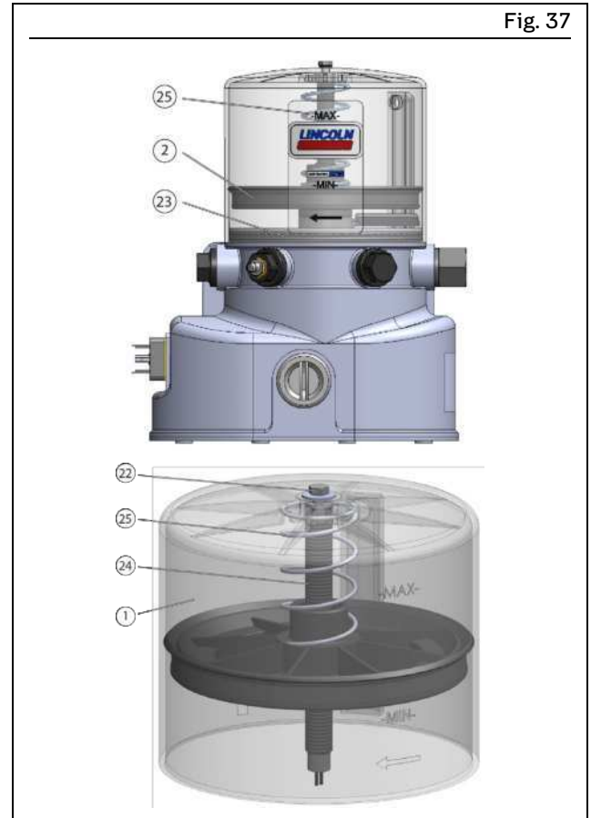
Replacing the follower plate
