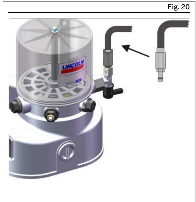
Installing the lubrication piping
