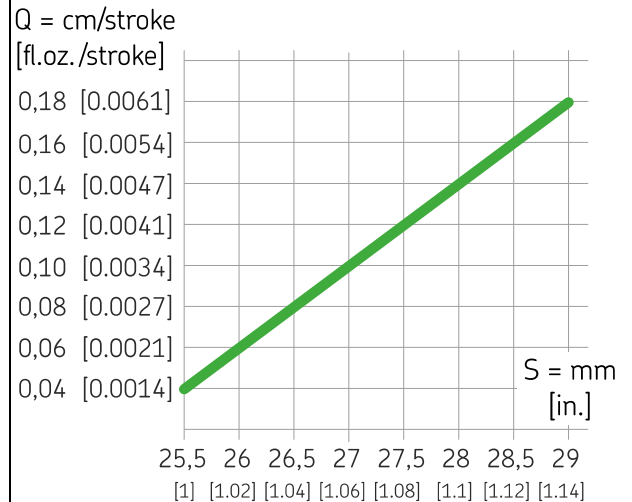
Delivery rate on pump element R or KR
