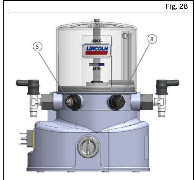
Initial filling of an empty pump without follower plate
