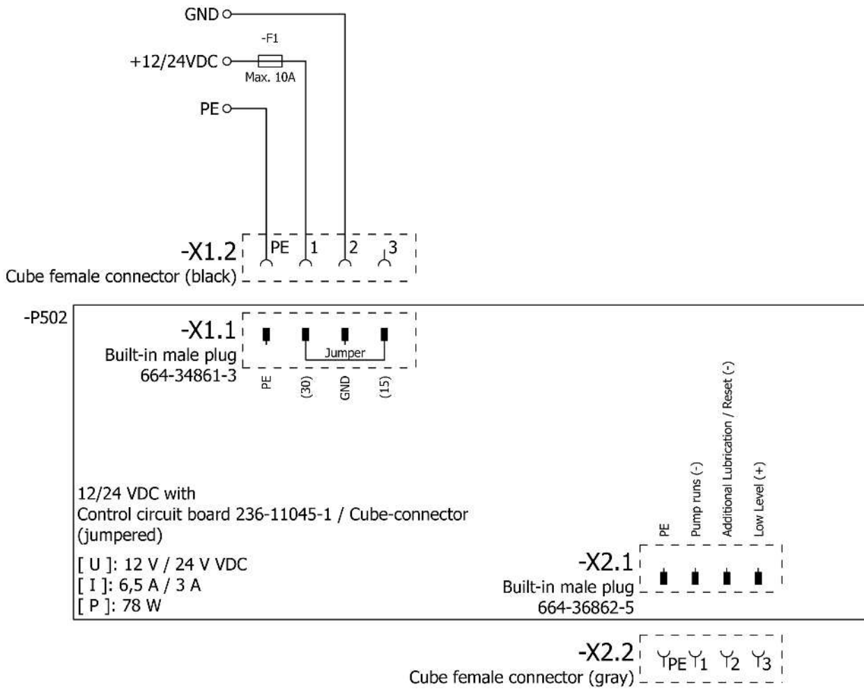
Terminal diagram 12 / 24 V DC with rectangular connector and control circuit board V10
