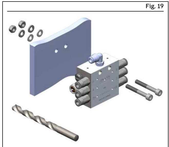
Installing the metering devices
