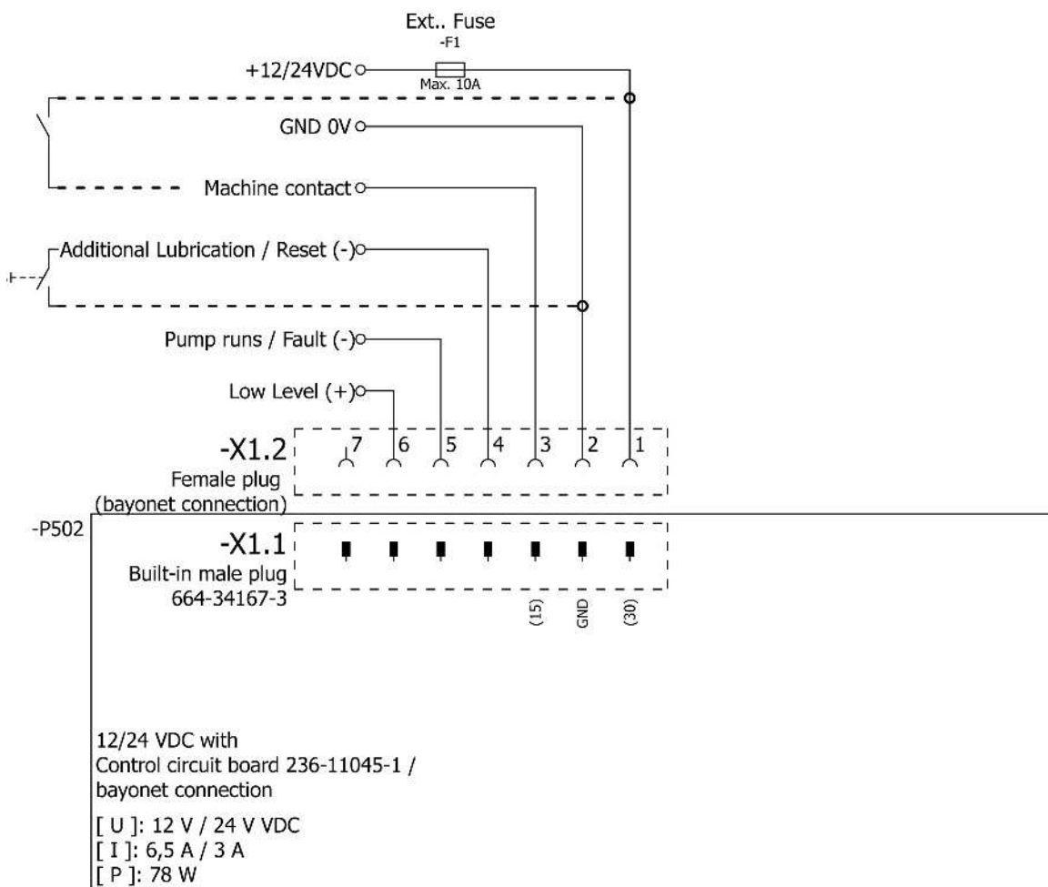
Terminal diagram 12 / 24 V DC with bayonet connector and control circuit board V20
