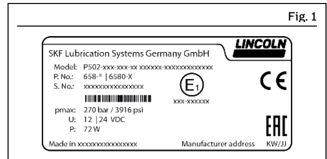
Type plate
