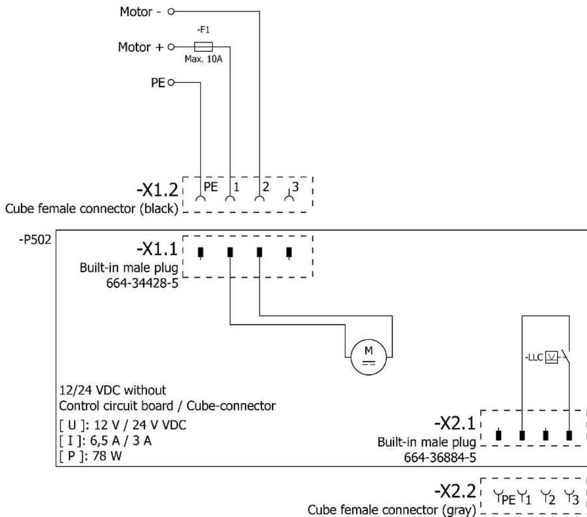
Terminal diagram 12 / 24 V DC with rectangular connector without control circuit board
