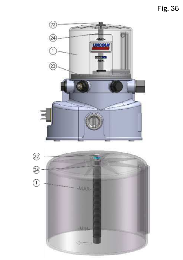
Replacing a reservoir without a follower plate
