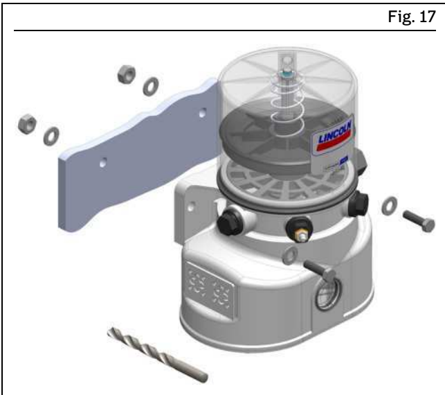
Installing the pump
