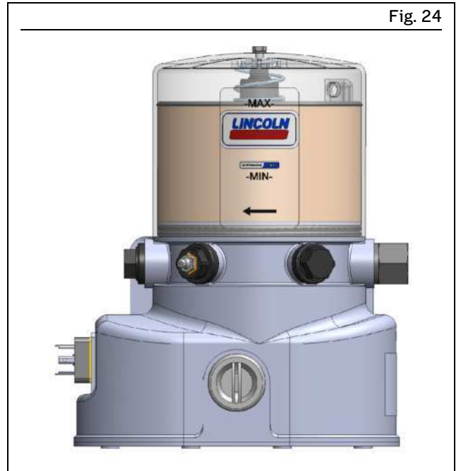
Pump filled and cable tie removed
