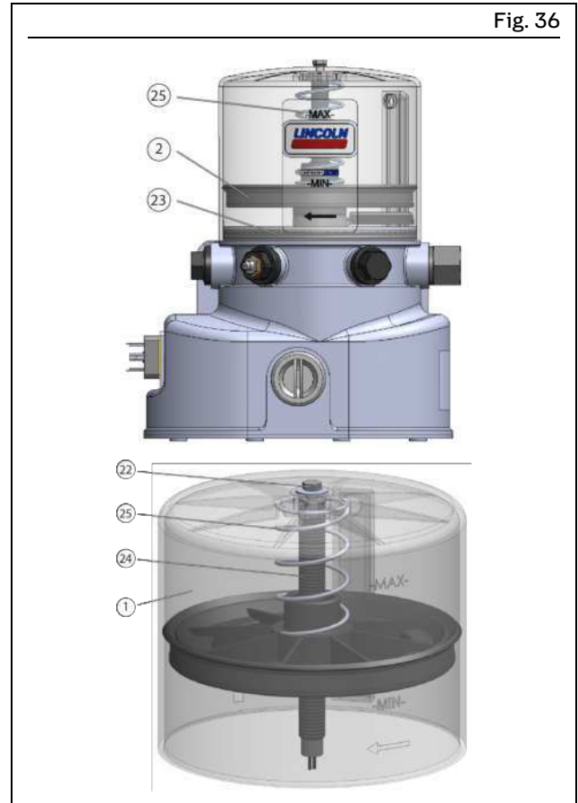
Replacing a reservoir with a follower plate (XLF)
