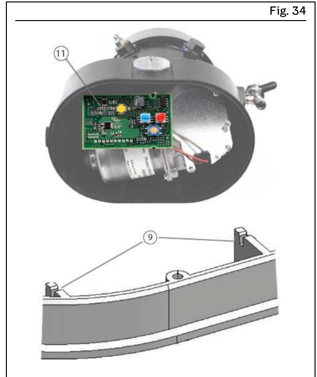
Replacing the control circuit board
