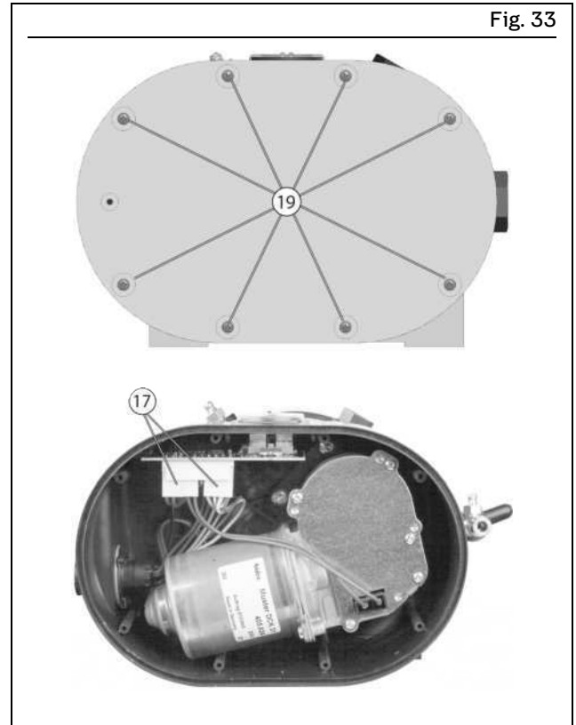
Replacing the control circuit board
